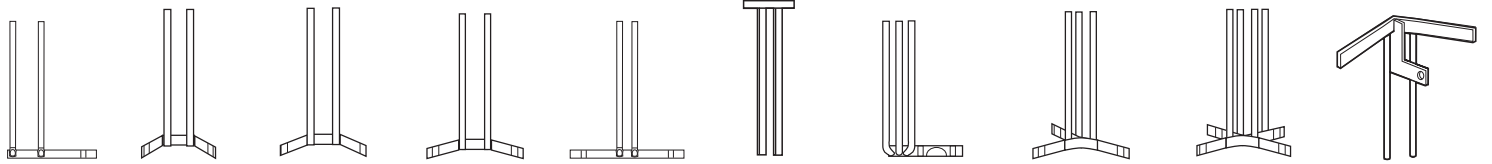
3000 U-connector, standard 3001 U-connector, triangle 60° 3002 U-connector, square 90° 3003 U-connector, hexagon 120° 3004 U-connector, 180° 3005 U-connector, side insert 3006 U-connector, 3-way cross 90° 3007 U-connector, 3-way cross 120° 3008 U-connector, 4-way cross 90° 3009 U-connector, with table top holder
