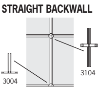
STRAIGHT BACKWALL
